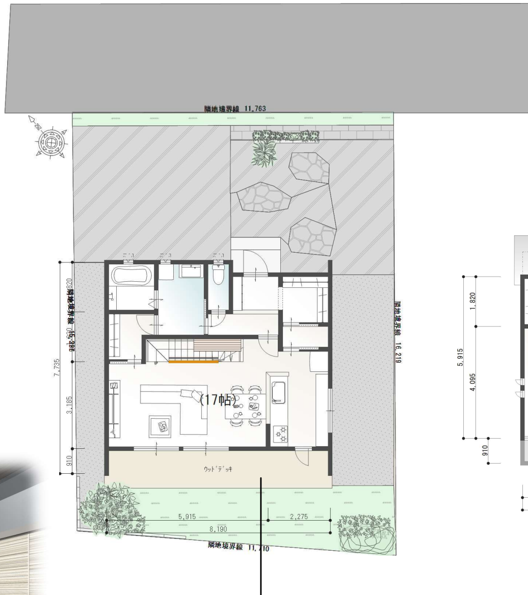
PLAN 1 F
